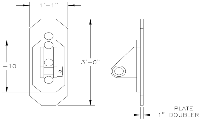
THUMB CYLINDER CLEVIS TO BE WELDED TO EXCAVATOR
