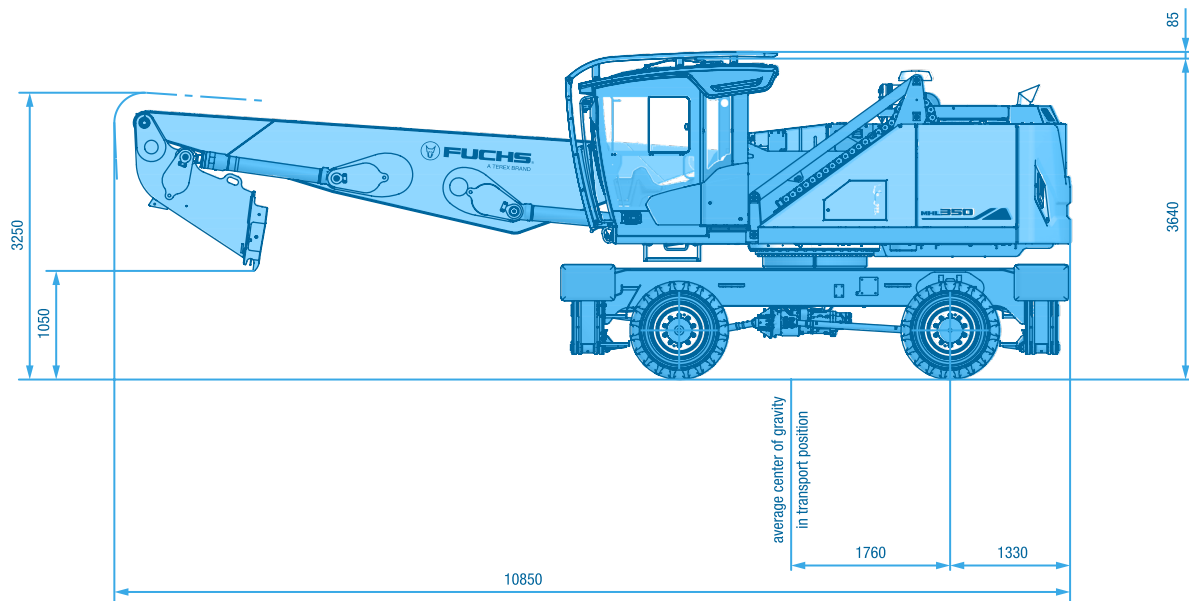
SIDE VIEW FQC (All dimensions in mm)
