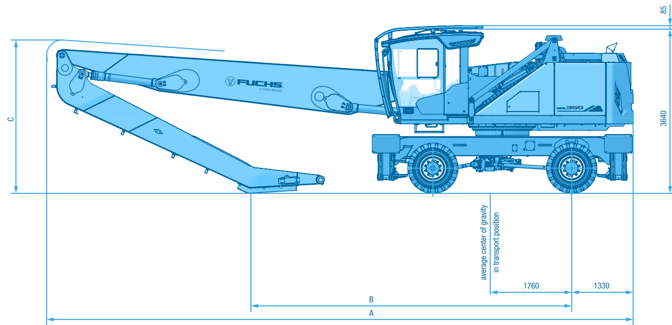
SIDE VIEW (All dimensions in mm)
