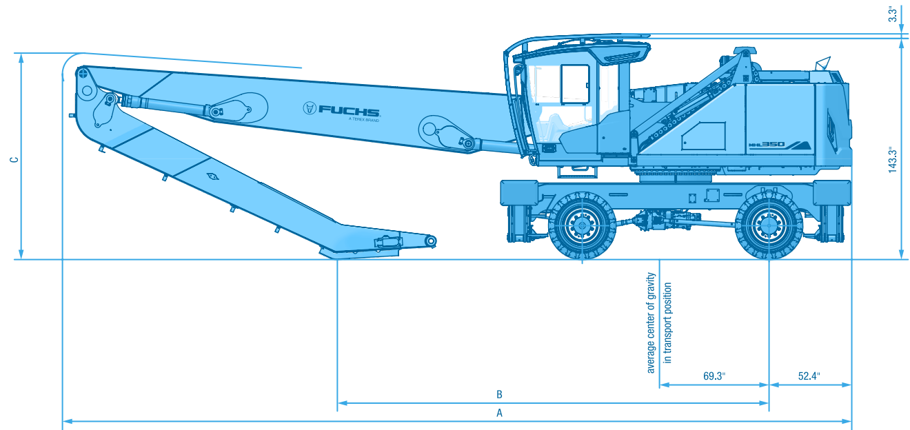
SIDE VIEW (All dimensions in ft and in)
