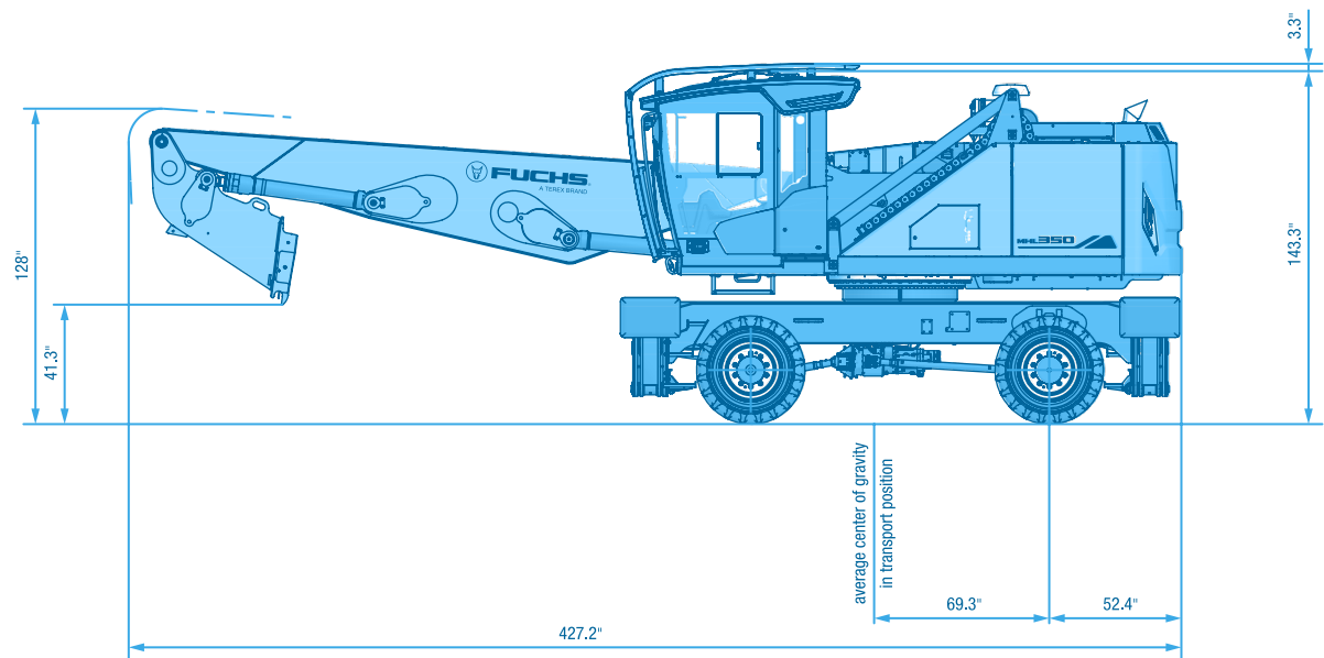
SIDE VIEW FQC (All dimensions in ft and in)
