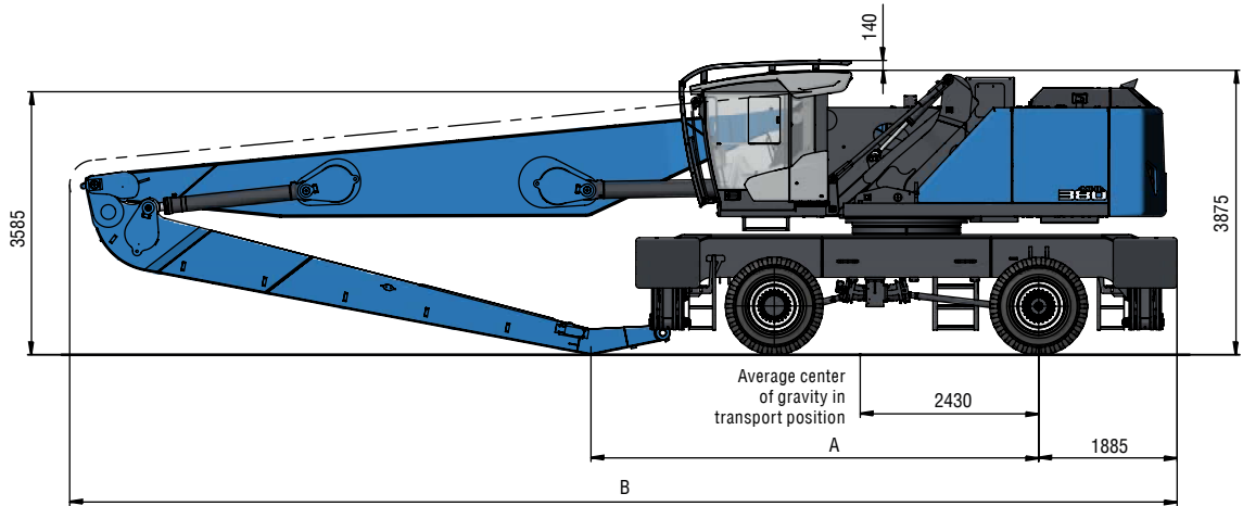
Loading equipment with dipper stick all dimensions in mm
