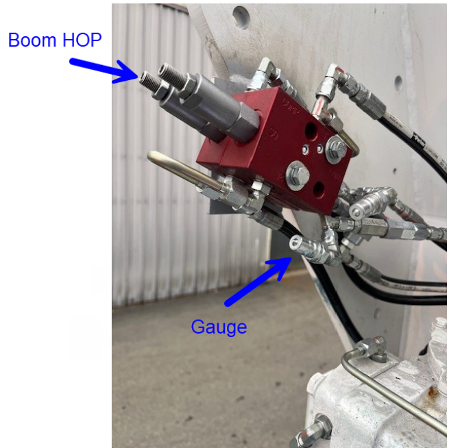
403835 HOP Boom Sensing Valve - Current
