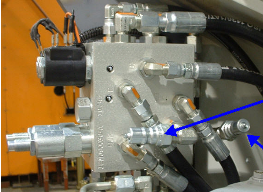
485770 HOP Manifold Shown for G1 Location (2006 units and newer)
