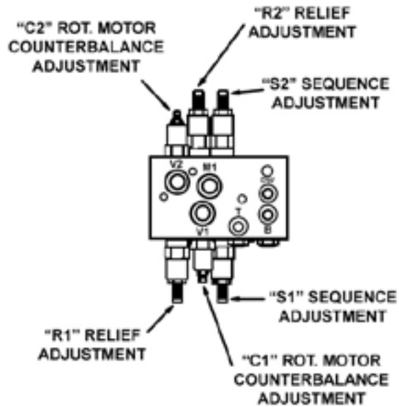
Old Valve Pre 1/1/2016
