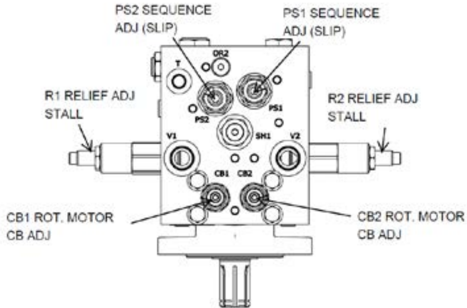
New Valve After 1/1/2016
