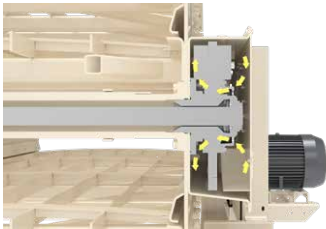
Cross-Section of Lubrication TSV6203
