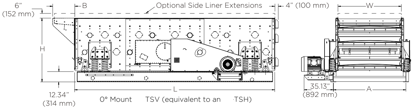
Dimension in inches (mm) for Standard Coil Springs **Subtract 1.25" (32 mm) for Optional Rubber Springs
