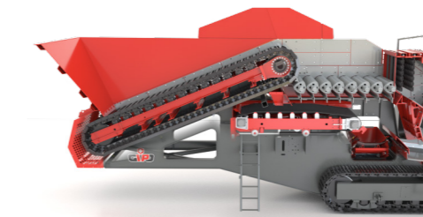
Apron feeder and roller grizzly
