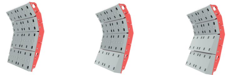
Impact plate design Single impact bar design Double impact bar design
