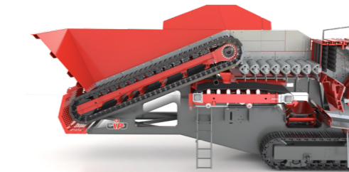
Apron feeder and roller grizzly
