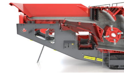
Integrated grizzly section
